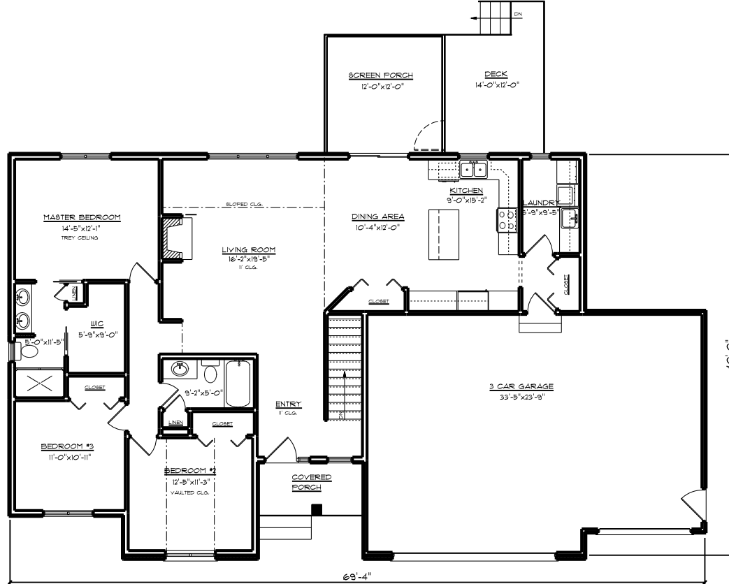
MAIN LEVEL FLOOR PLAN MAIN LEVEL SQ. FT.: 1625 SQ. FT. TOTAL FINISHED SQ. FT.: 1625 SQ. FT.
