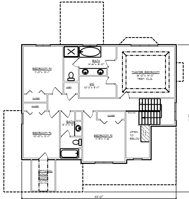
UPPER LEVEL FLOOR PLAN
